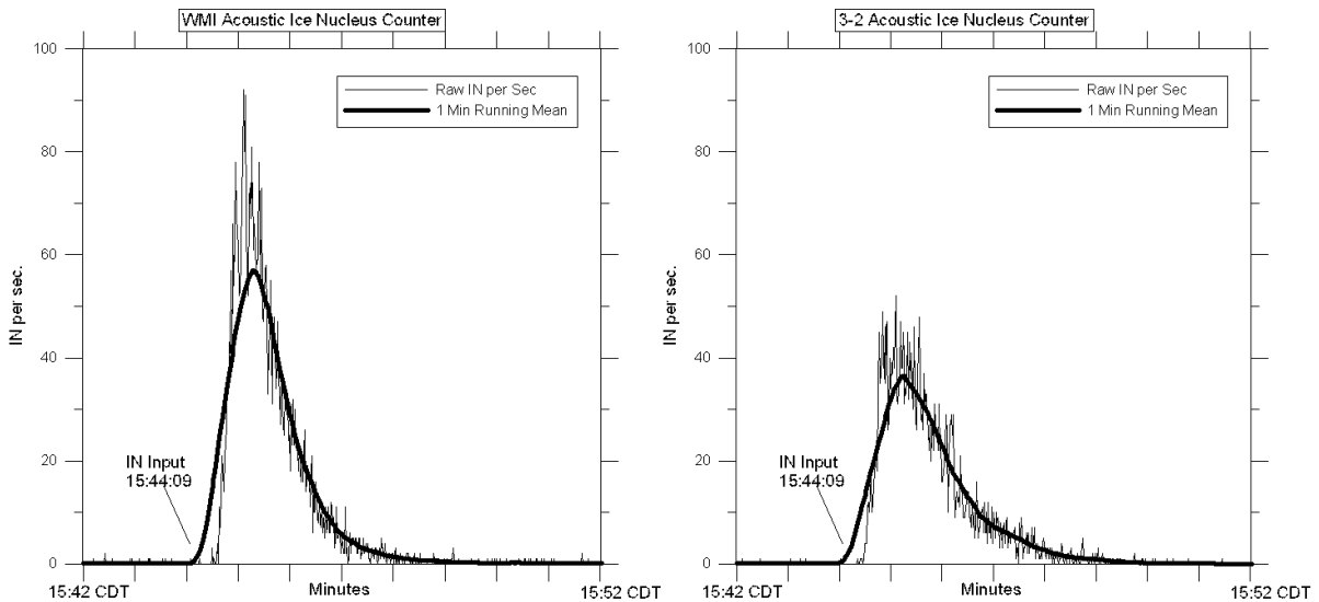
Fig. 1. Plots of detected IN from combustion of AgI-NH 4 I-acetone solution on a match. Both 1 s accumulations of IN and 1 min running means are shown. The left graph is for the WMI AINC and the right for Unit 3-2. The period corresponds to the middle plume in Fig. 2.
