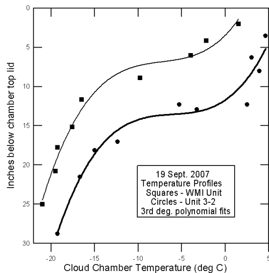
Fig. 4. Vertical temperature profiles of the two AINC chambers taken approximately 1 inch from the cloud chamber wall. The curves are cubic fits to the data.
